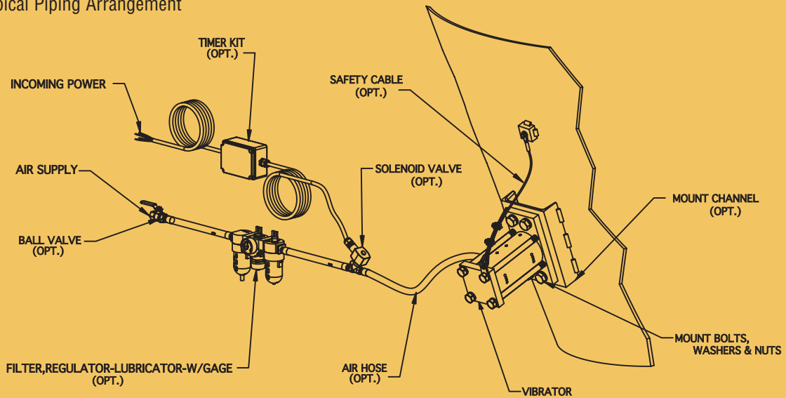
Typical Piping Arrangement
