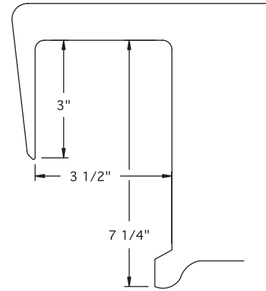
Attaching Head Detail
